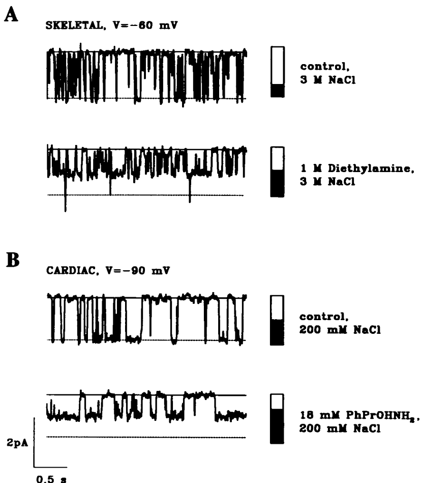
FIGURE 4 (A) Traces recorded from a BTX-activated rat skeletal muscle sodium channel. In this particular experiment, the recording solution was 3 M NaCl/50 mM MOPS at a pH of 7.0. In absence of blockers, this channel was closed most of the time at a membrane potential of -60 mV. Perfusion of the chamber facing the intracellular side of the channel with 1 M diethylamine in 3 M NaCl/50 mM MOPS resulted in pronounced block and a pronounced increase in open probability. The three downward deflections in the diethylamine trace reflect bilayer instability, not opening of a second channel. (B) Current traces recorded from a BTX-activated bovine cardiac sodium channel, bathed in symmetric 200 mM NaCl/20 mM MOPS (pH 7.0), at a membrane potential of -90 mV. As in Fig. 2, application of 18 mM phenylpropanolamine caused fast block and an increase in apparent open probability. For both panels A and B, solid lines superimposed on the records indicate the closed level, and the dashed lines indicate the open level in absence of blockers. All records were filtered at 50 Hz. The solid bars to the right of the traces reflect the apparent open probability on a scale from 0 to 1.
